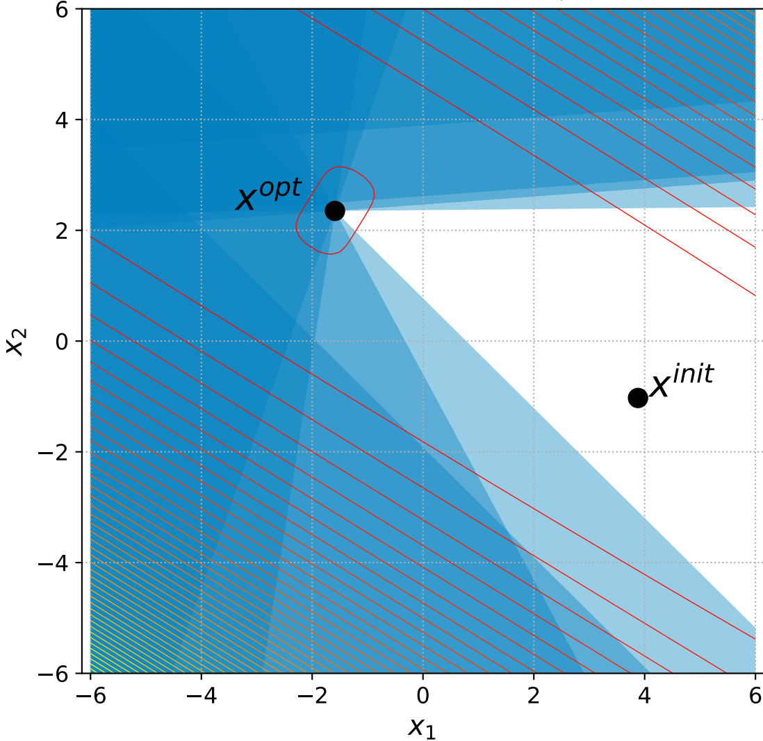
39 Different Powers with 6 constraints, instance=11
