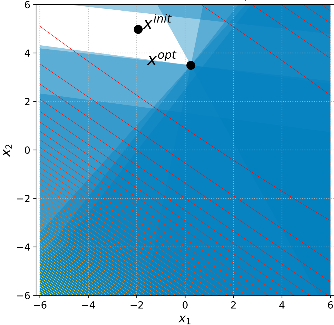
39 Different Powers with 6 constraints, instance=10
