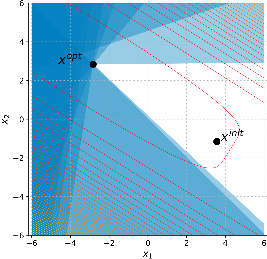
39 Different Powers with 6 constraints, instance=6
