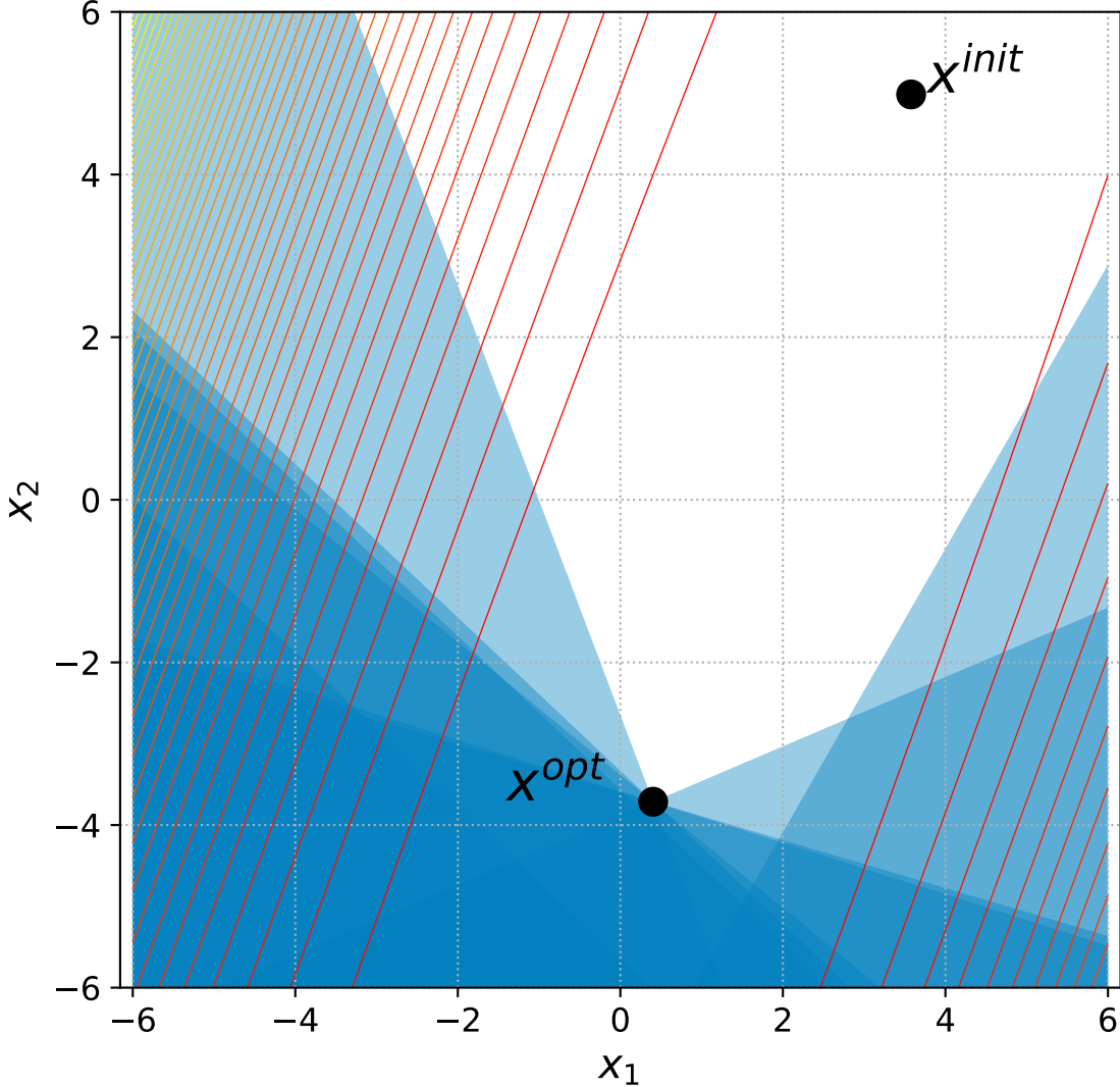
39 Different Powers with 6 constraints, instance=4
