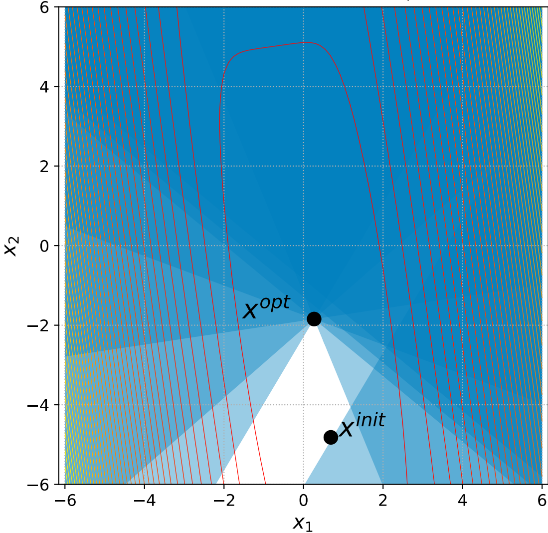
39 Different Powers with 6 constraints, instance=3
