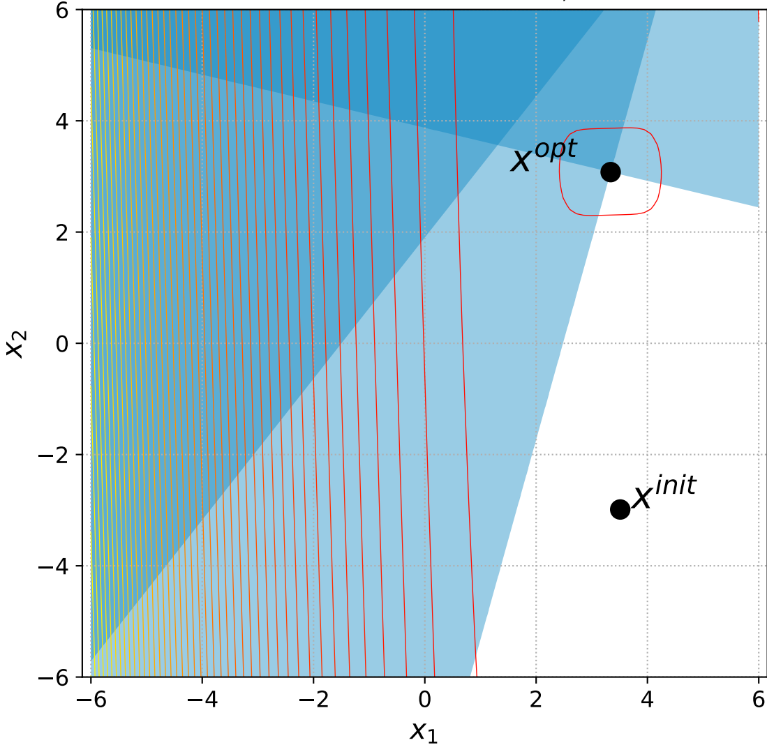
38 Different Powers with 2 constraints, instance=15
