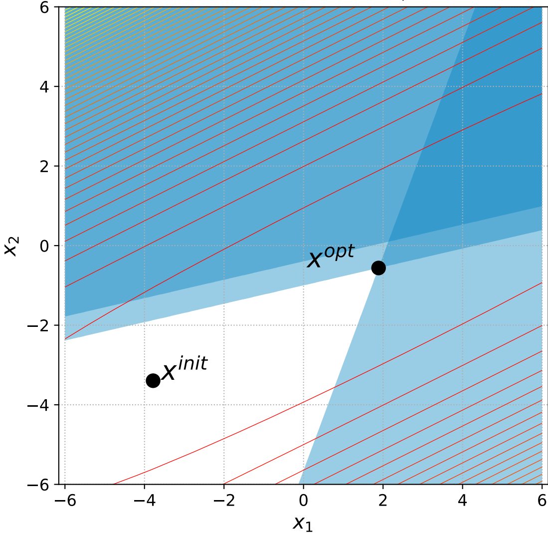
38 Different Powers with 2 constraints, instance=12
