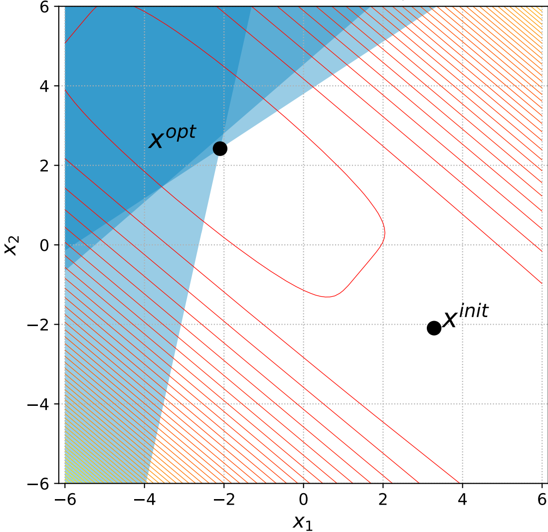
38 Different Powers with 2 constraints, instance=11
