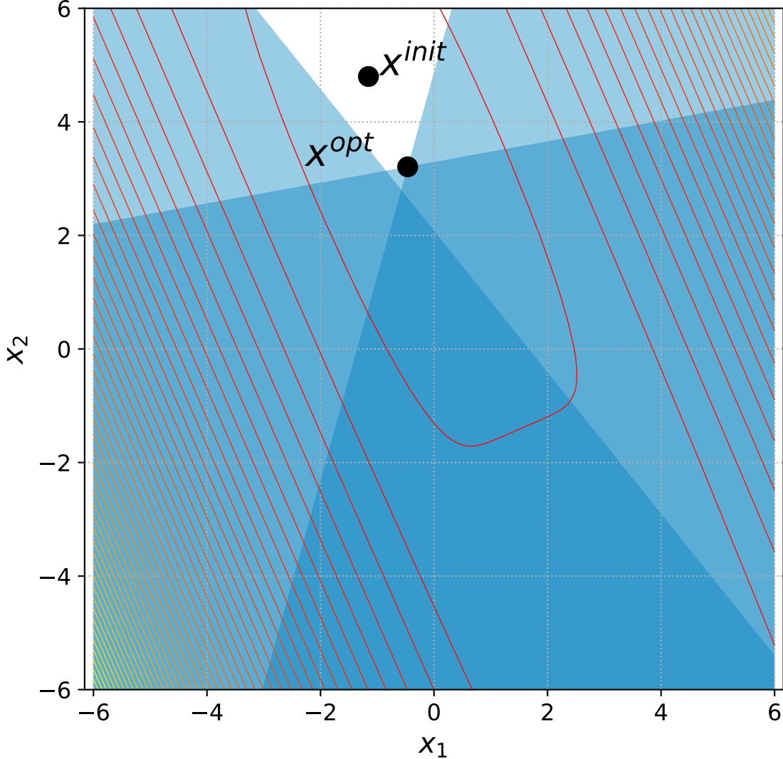
38 Different Powers with 2 constraints, instance=10
