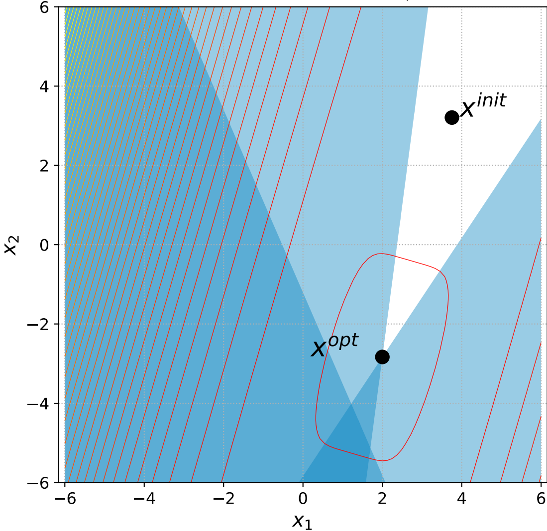
38 Different Powers with 2 constraints, instance=9
