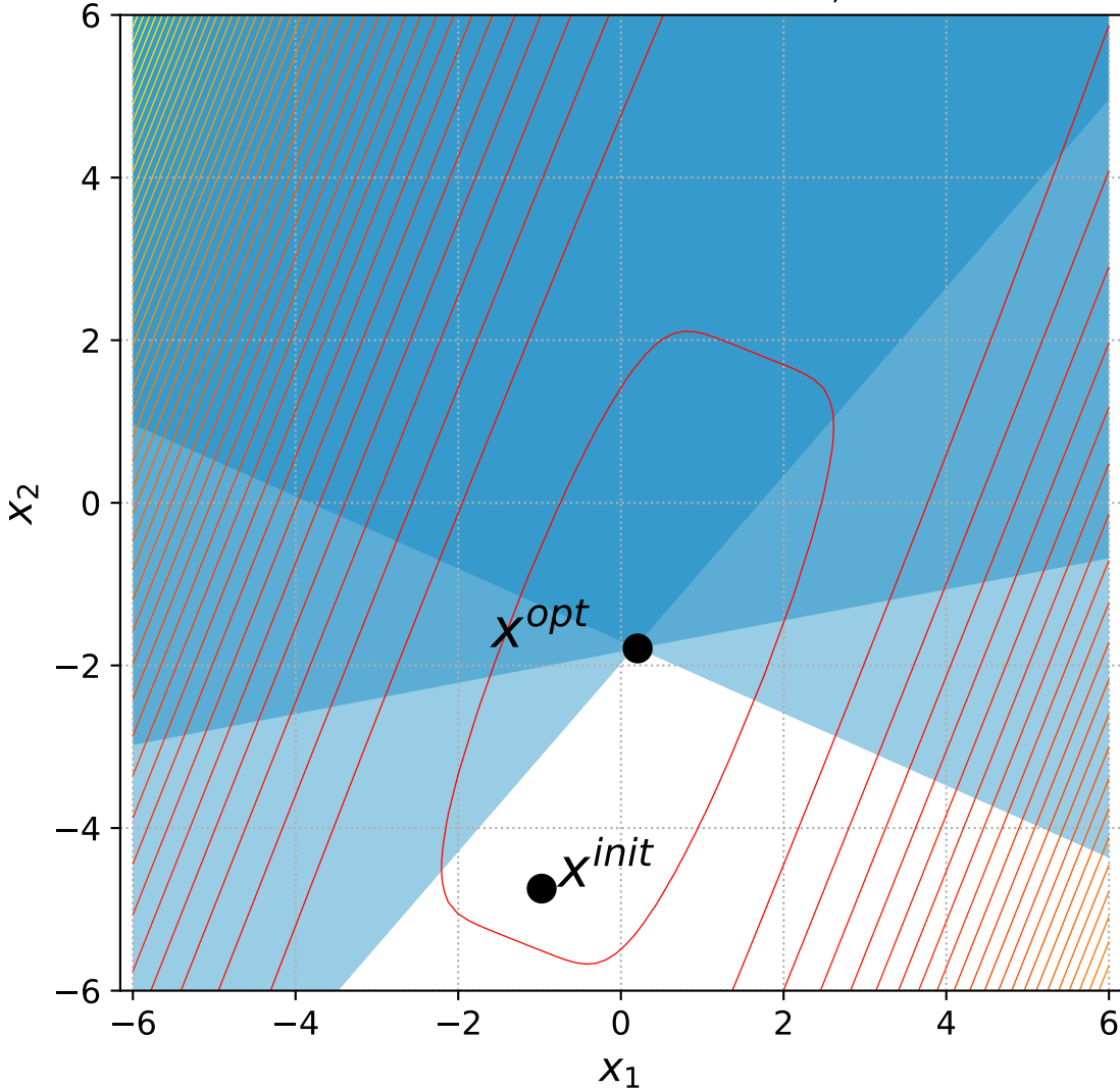
38 Different Powers with 2 constraints, instance=8
