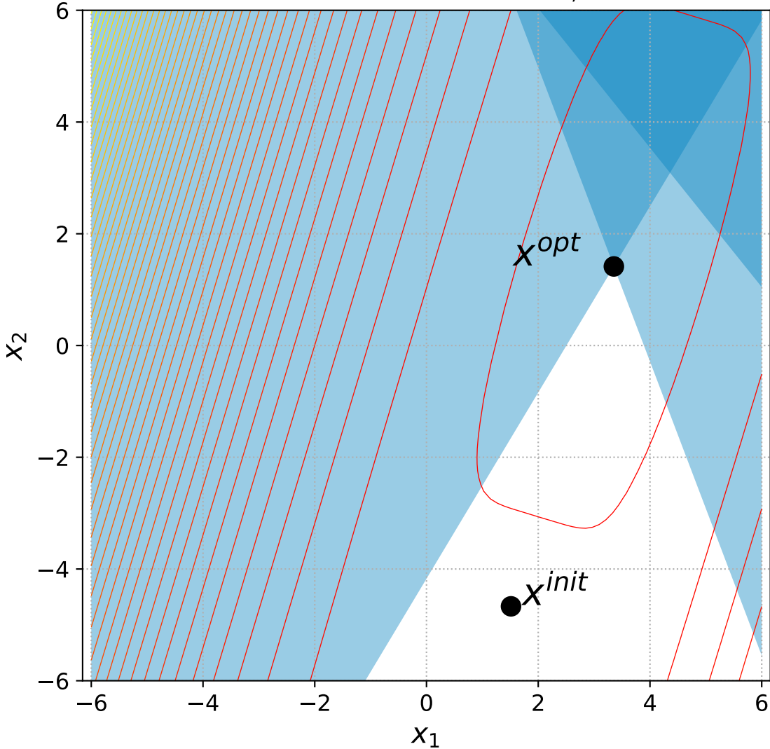
38 Different Powers with 2 constraints, instance=5
