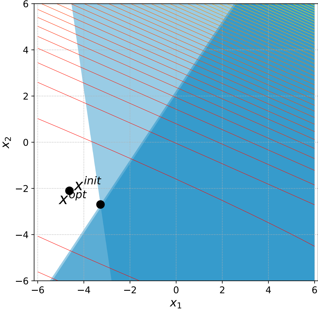
38 Different Powers with 2 constraints, instance=4
