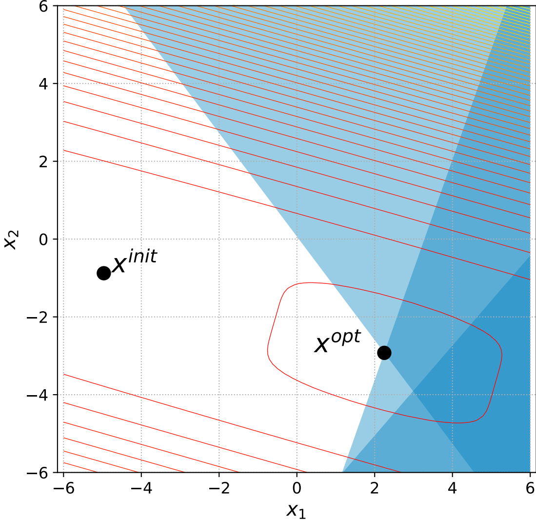
38 Different Powers with 2 constraints, instance=3
