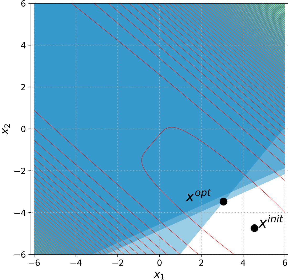
38 Different Powers with 2 constraints, instance=2
