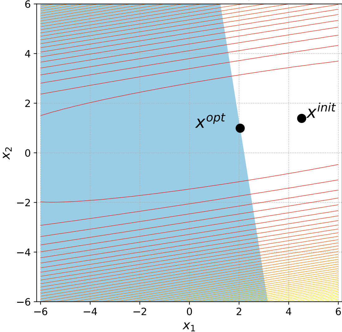
37 Different Powers with 1 constraint, instance=13
