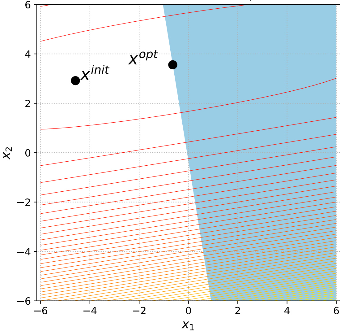
37 Different Powers with 1 constraint, instance=7
