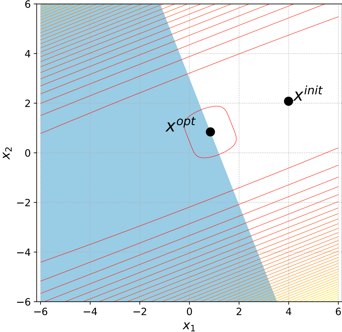
37 Different Powers with 1 constraint, instance=6
