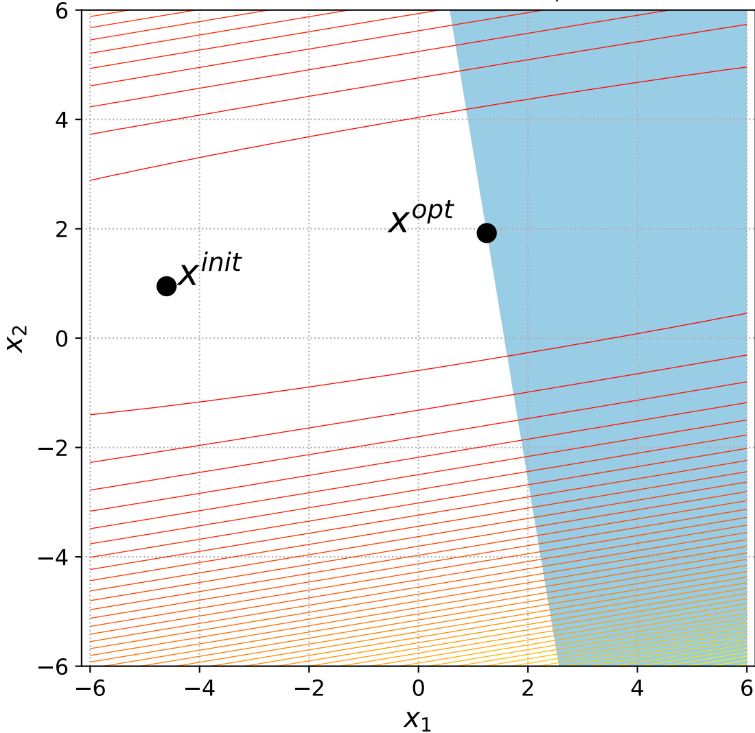
37 Different Powers with 1 constraint, instance=3
