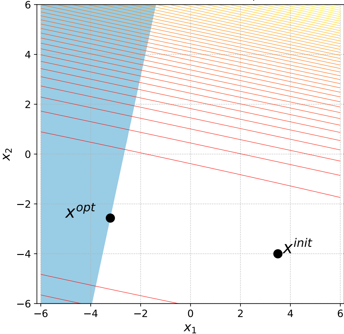
37 Different Powers with 1 constraint, instance=2
