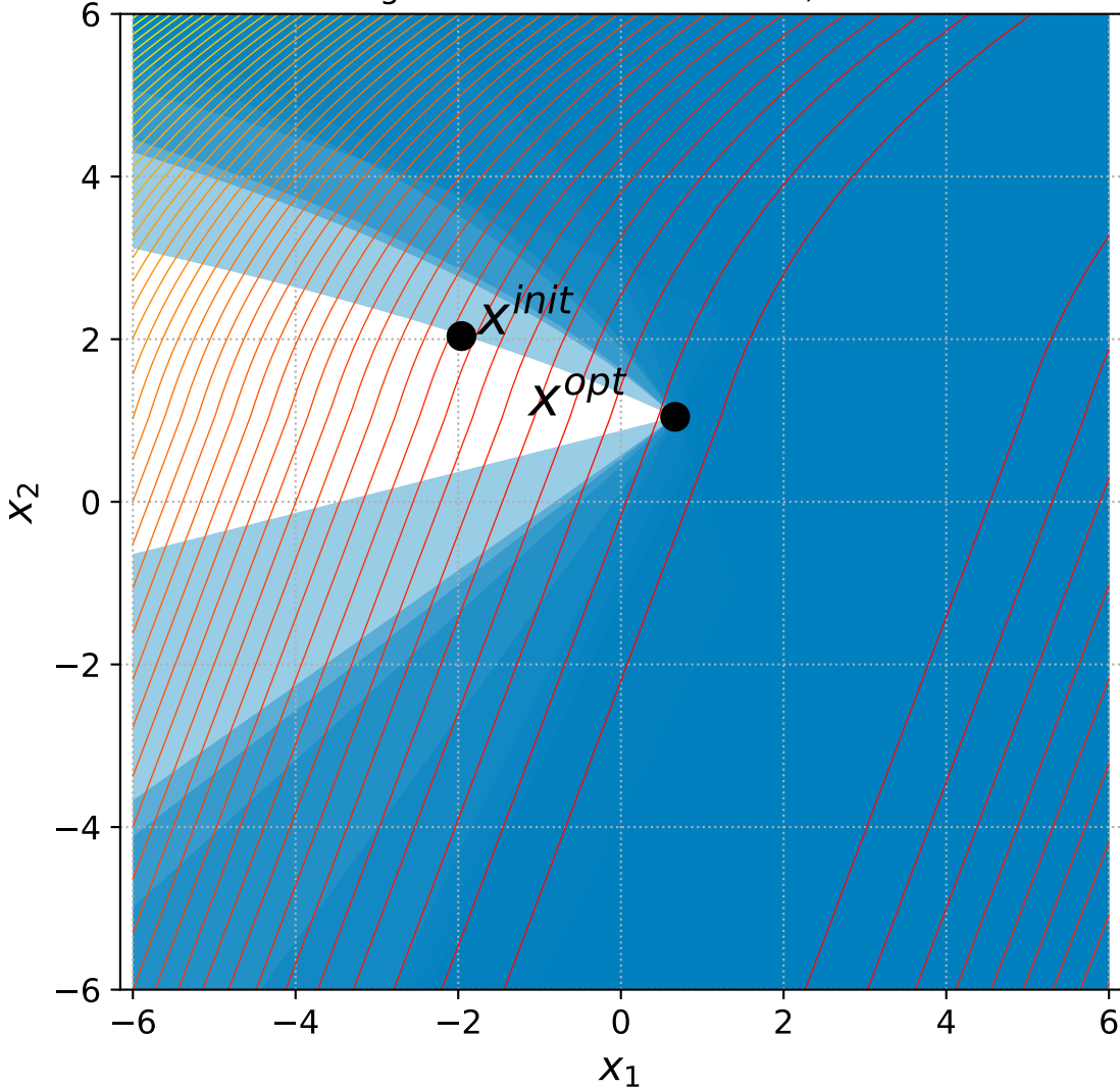
36 Bent Cigar with 6+3n constraints, instance=15
