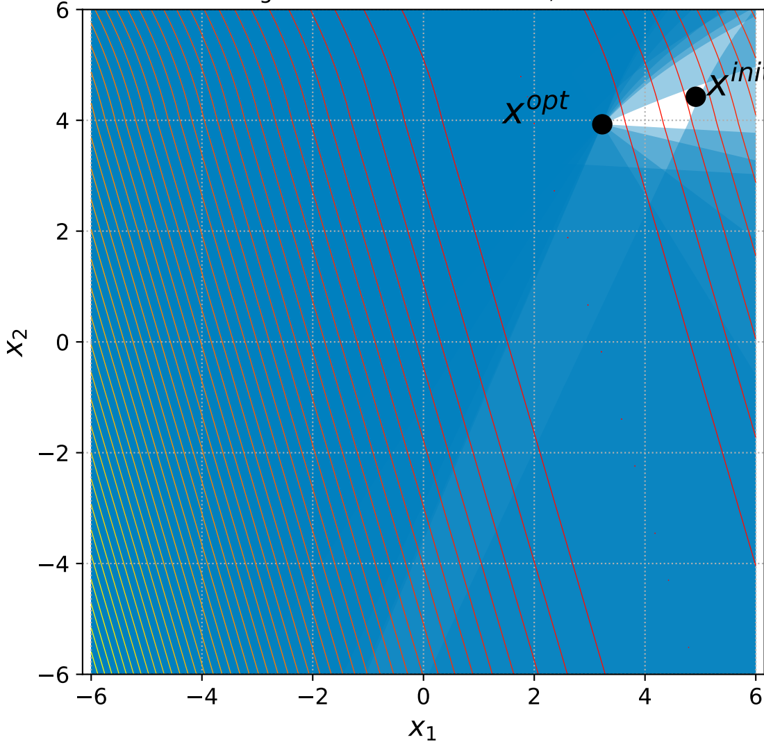
36 Bent Cigar with 6+3n constraints, instance=14
