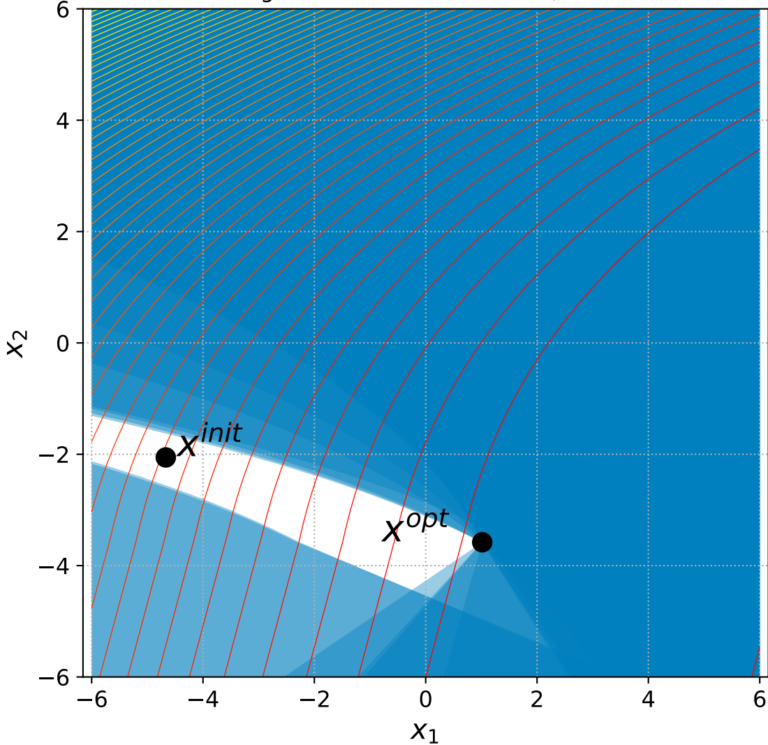
36 Bent Cigar with 6+3n constraints, instance=11
