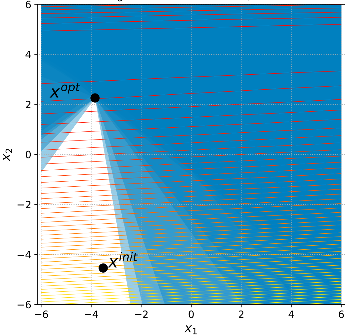
36 Bent Cigar with 6+3n constraints, instance=10
