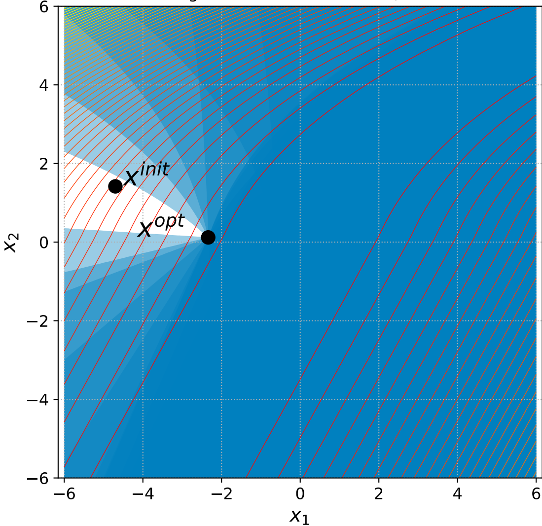
36 Bent Cigar with 6+3n constraints, instance=9
