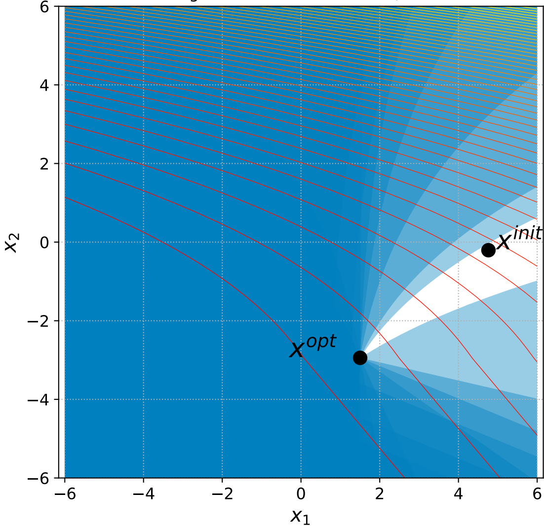
36 Bent Cigar with 6+3n constraints, instance=8
