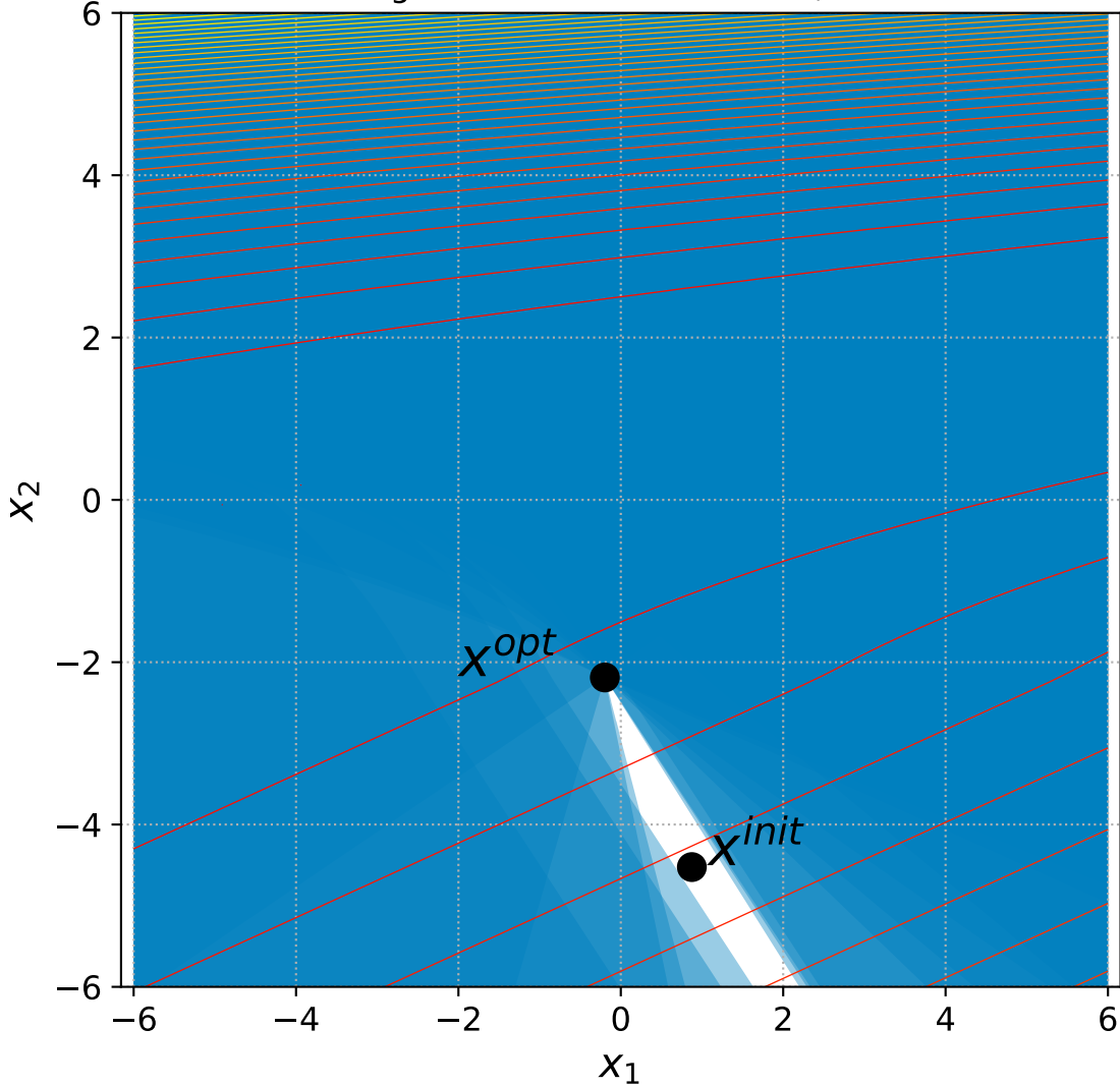
36 Bent Cigar with 6+3n constraints, instance=6
