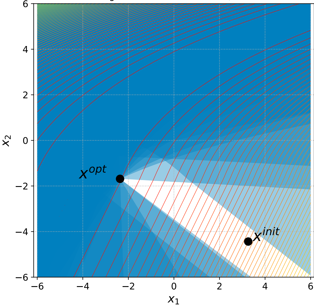
36 Bent Cigar with 6+3n constraints, instance=4
