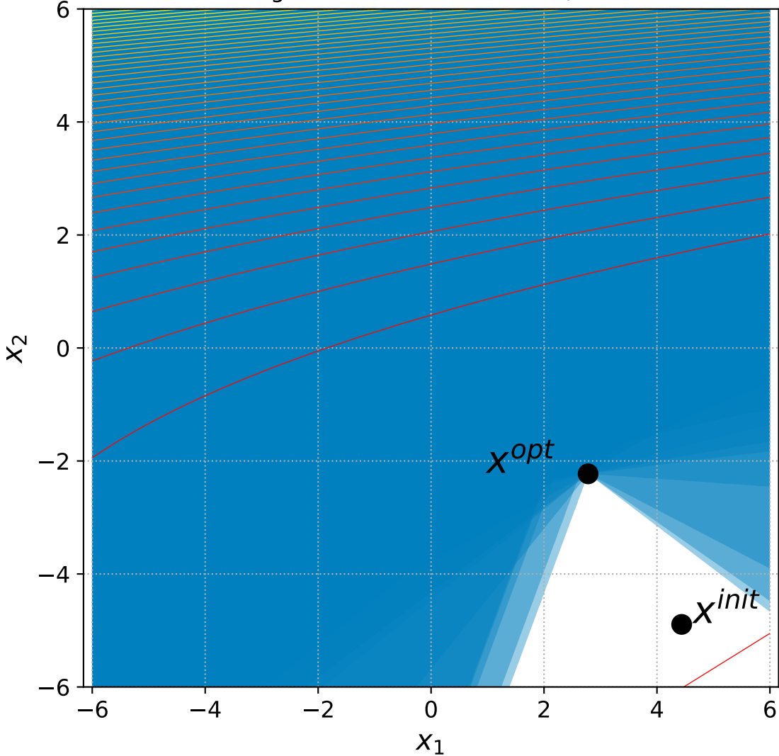
36 Bent Cigar with 6+3n constraints, instance=2
