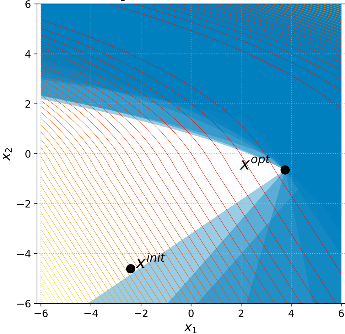
36 Bent Cigar with 6+3n constraints, instance=1
