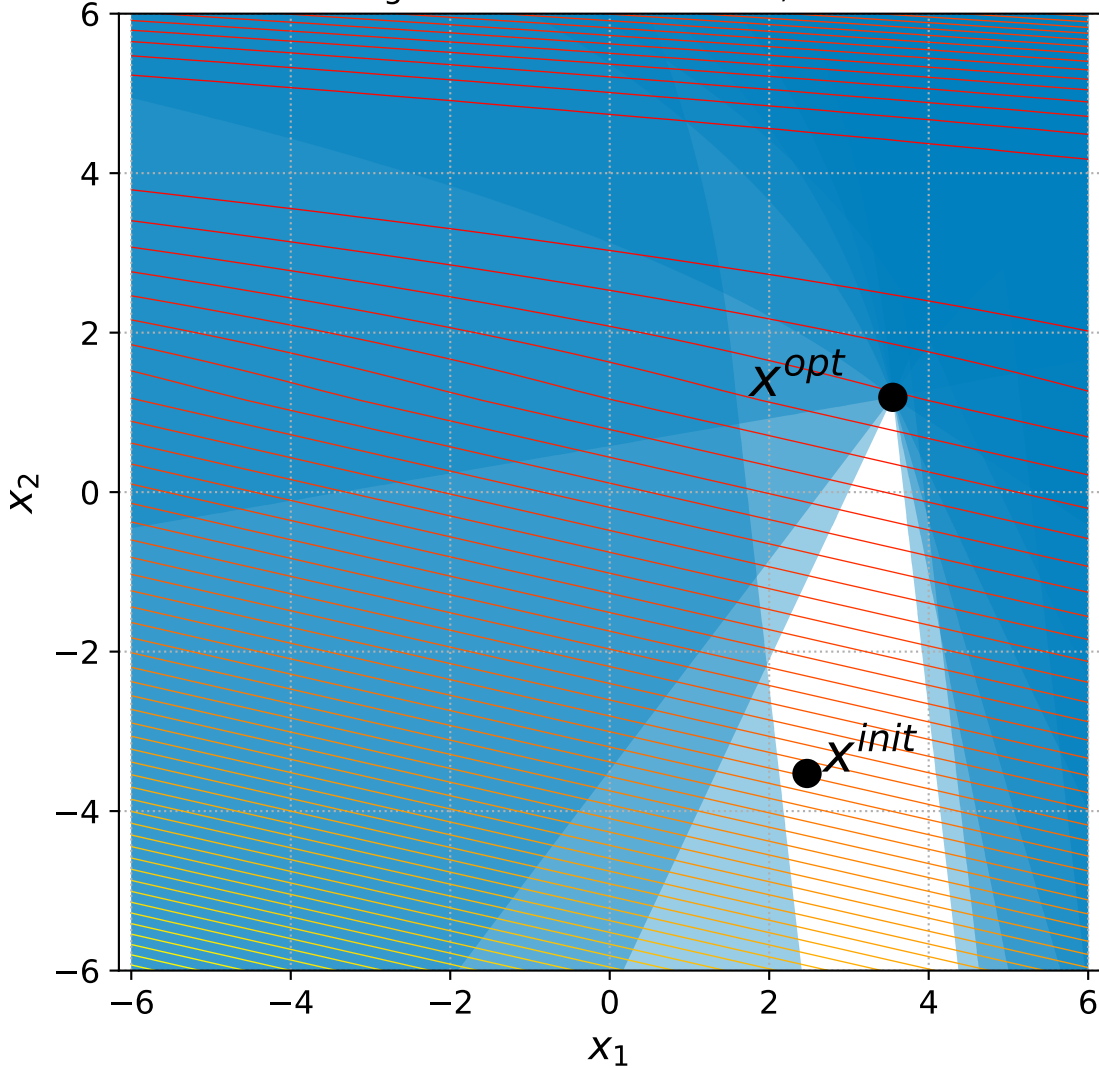
35 Bent Cigar with 6+n constraints, instance=15
