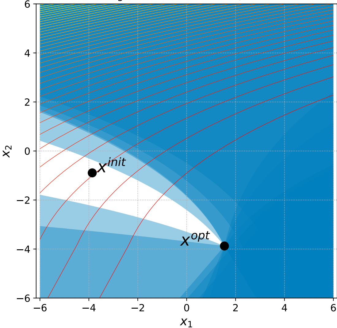
35 Bent Cigar with 6+n constraints, instance=14
