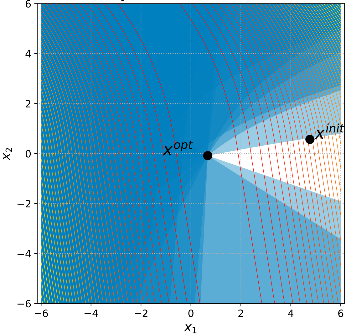
35 Bent Cigar with 6+n constraints, instance=13
