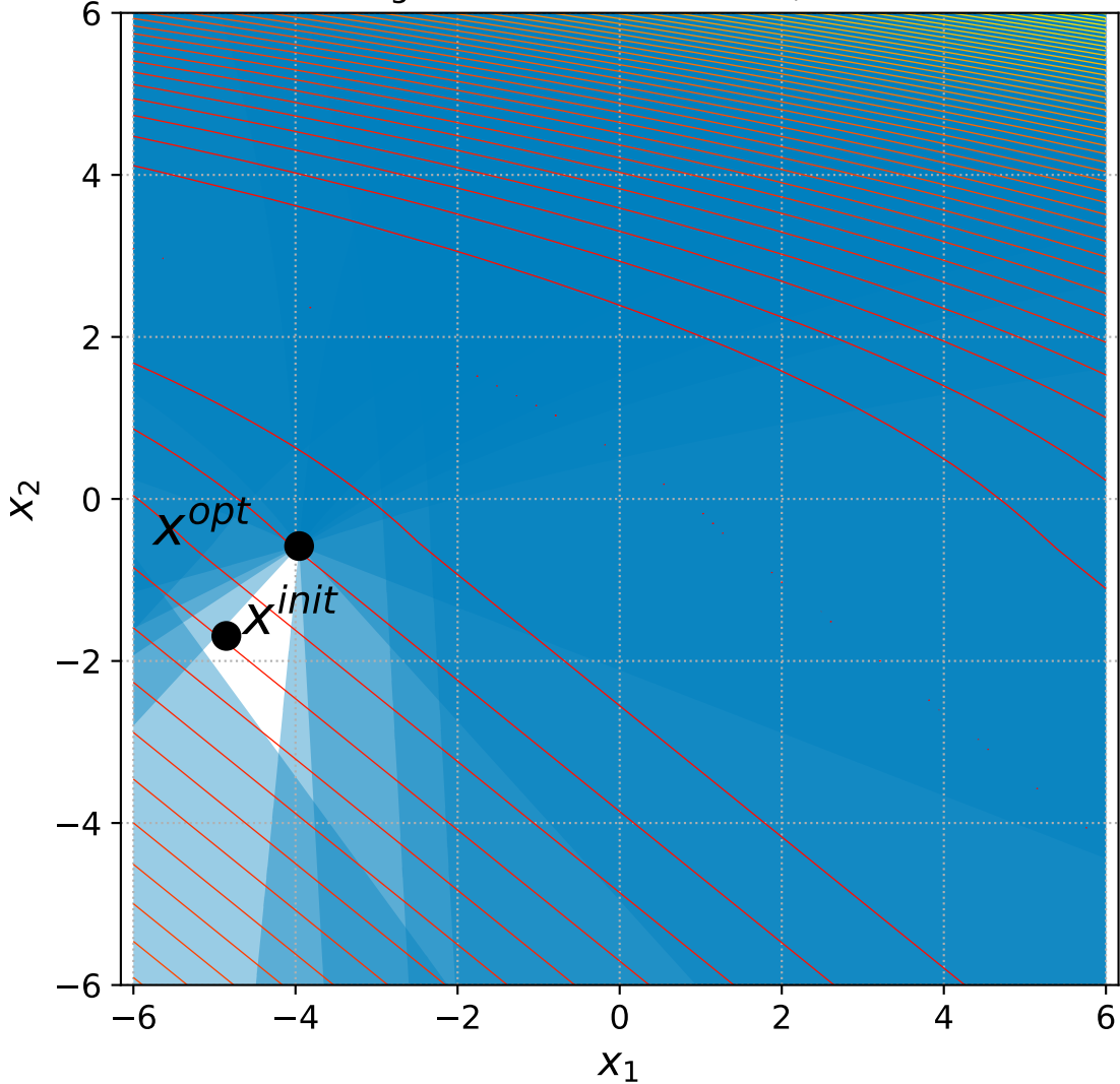
35 Bent Cigar with 6+n constraints, instance=12
