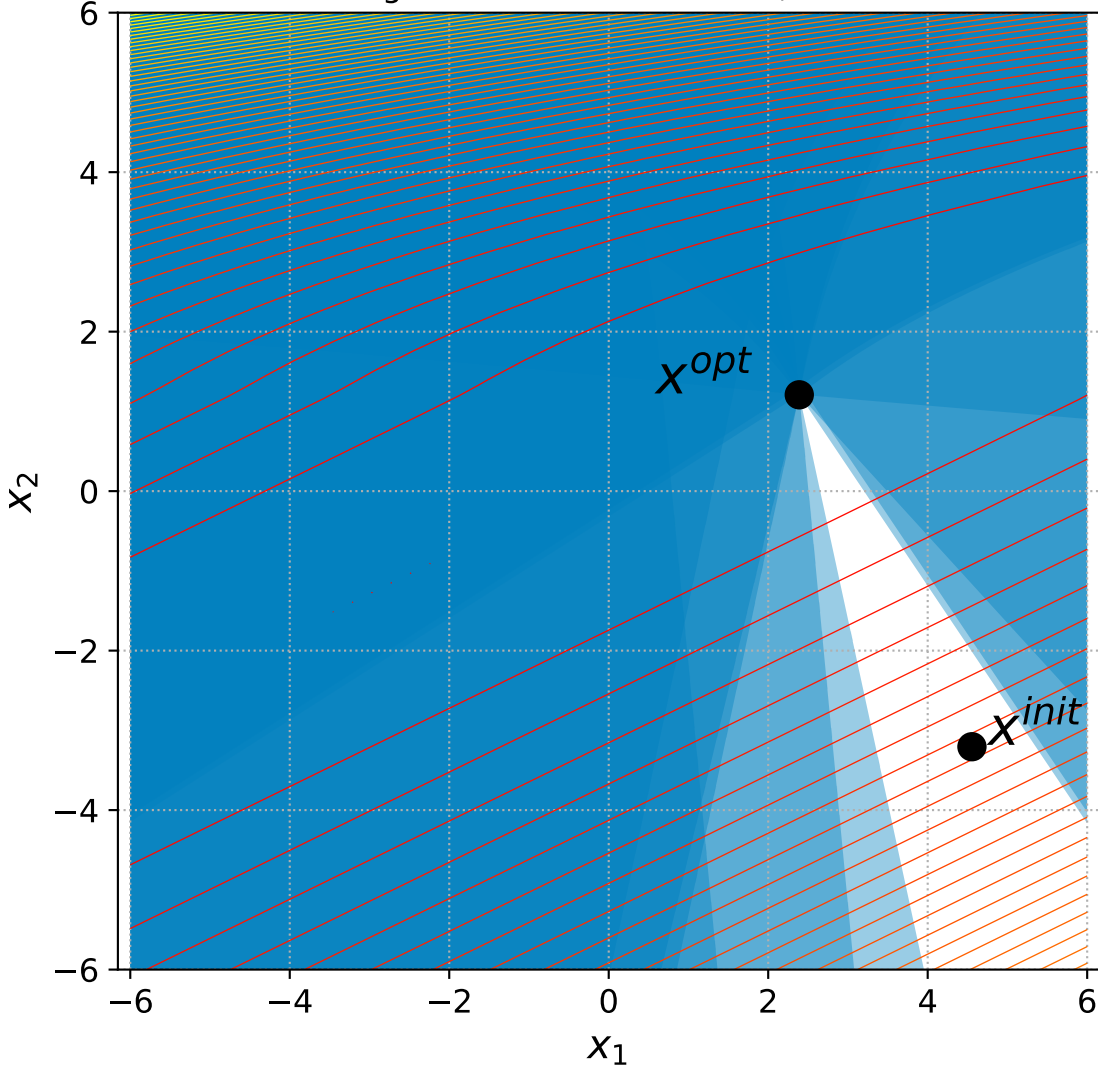
35 Bent Cigar with 6+n constraints, instance=11
