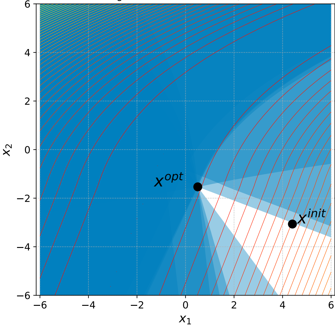
35 Bent Cigar with 6+n constraints, instance=10
