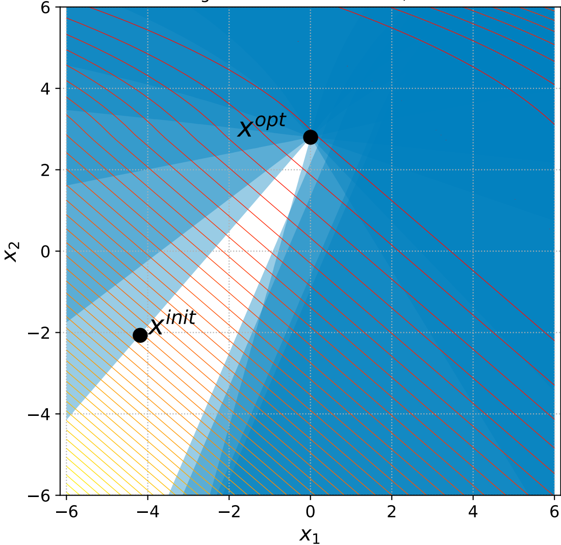
35 Bent Cigar with 6+n constraints, instance=9
