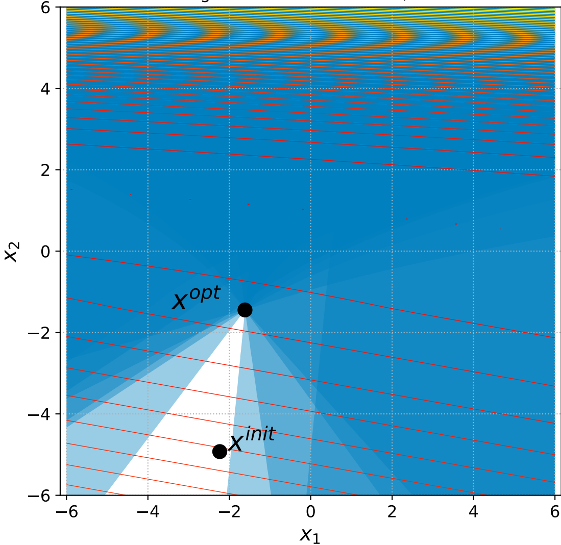
35 Bent Cigar with 6+n constraints, instance=7
