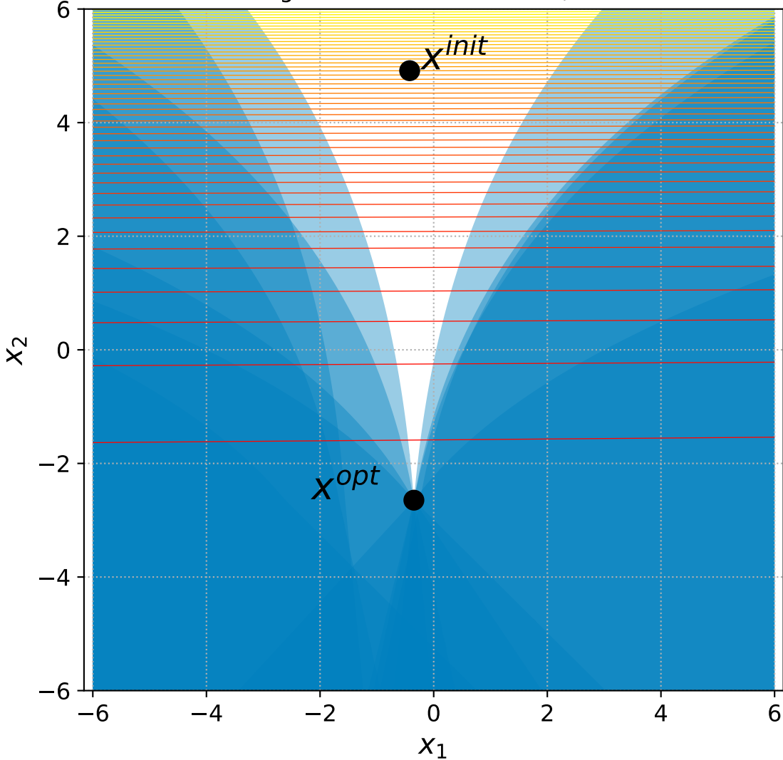
35 Bent Cigar with 6+n constraints, instance=6
