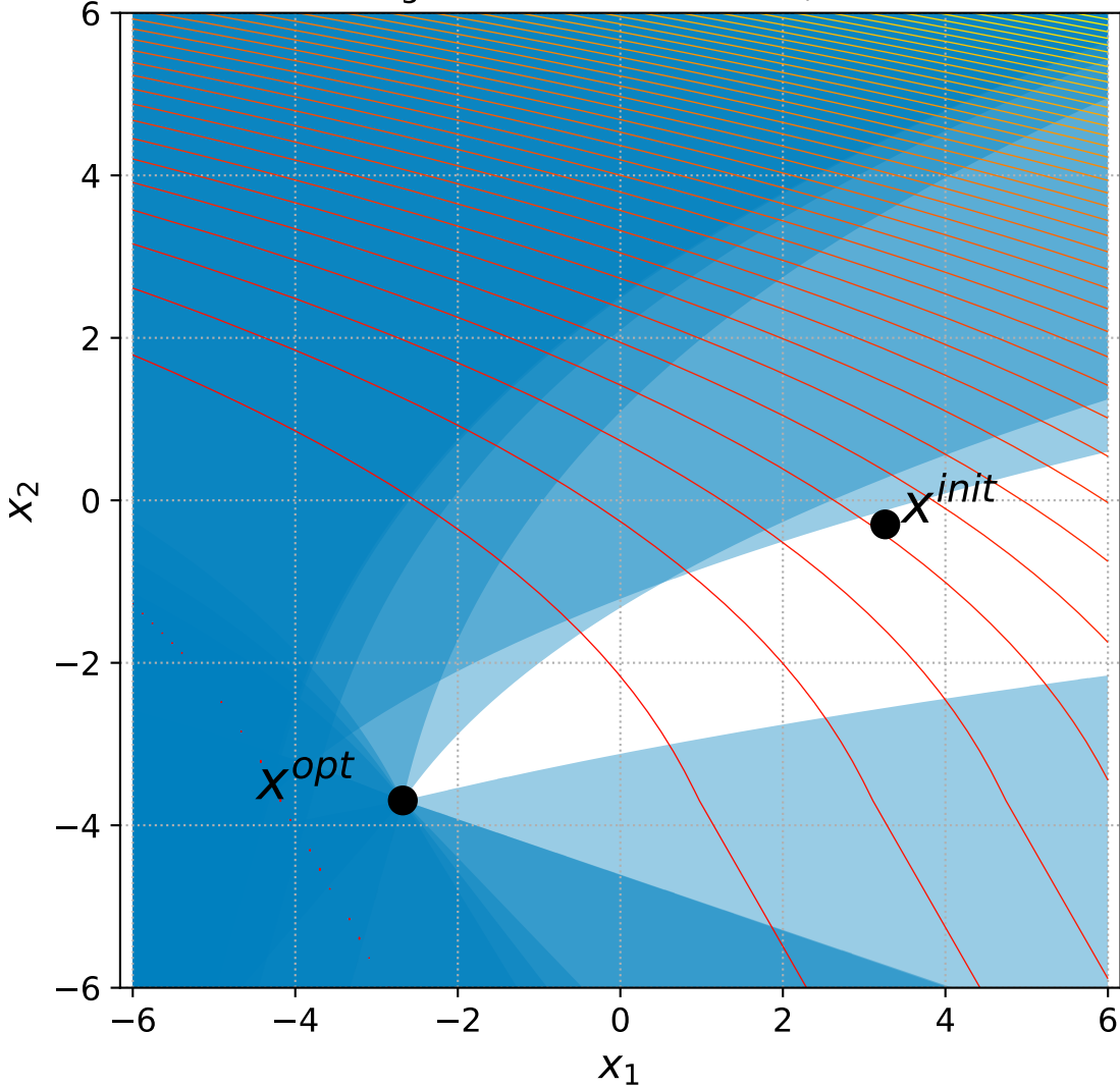
35 Bent Cigar with 6+n constraints, instance=4
