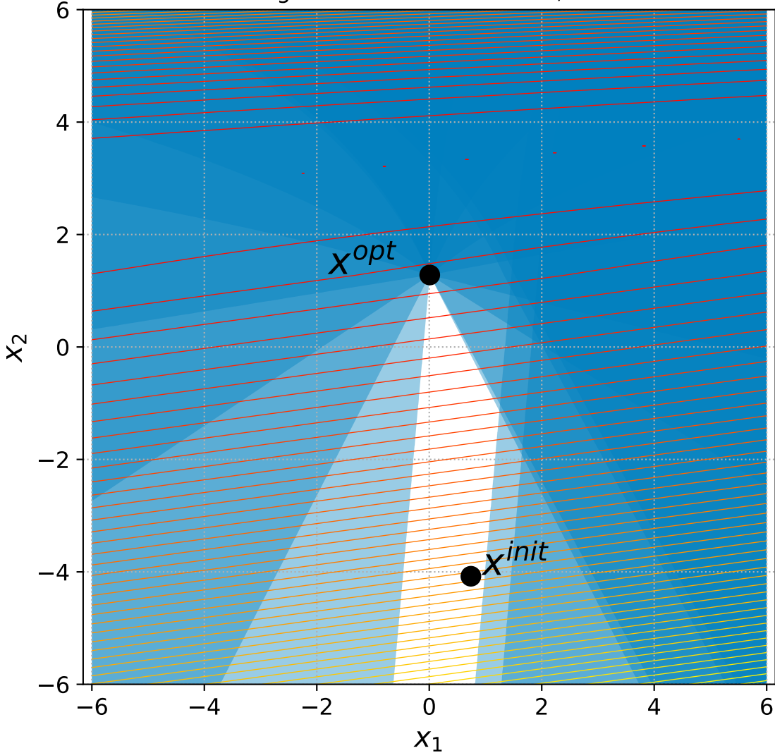
35 Bent Cigar with 6+n constraints, instance=3
