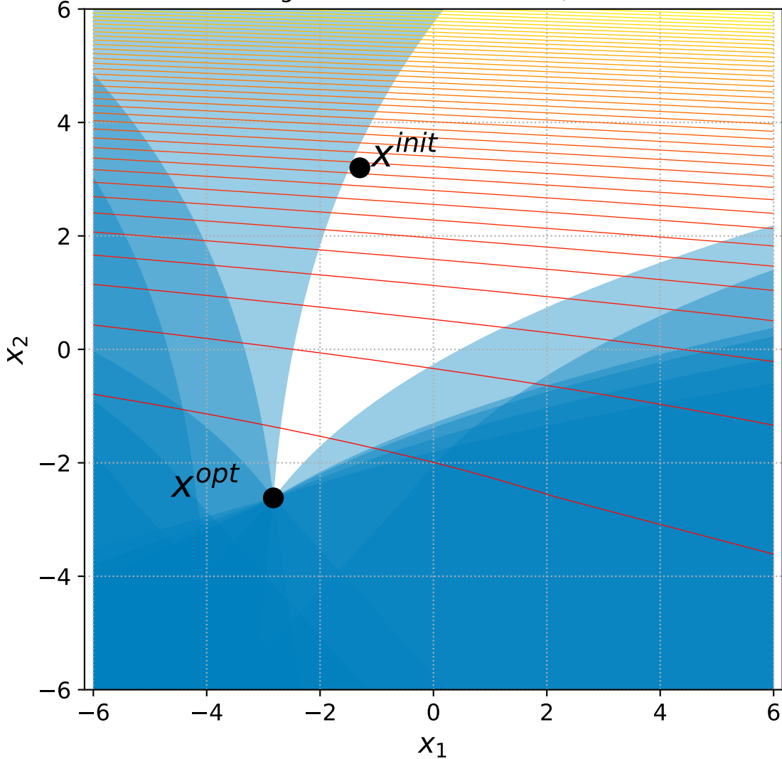
35 Bent Cigar with 6+n constraints, instance=2
