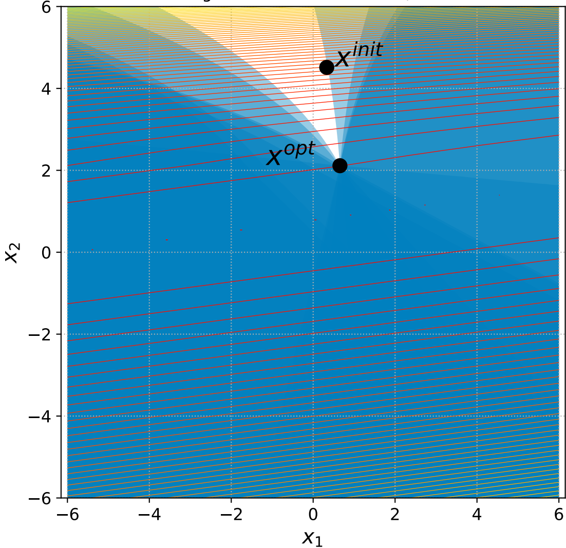
35 Bent Cigar with 6+n constraints, instance=1
