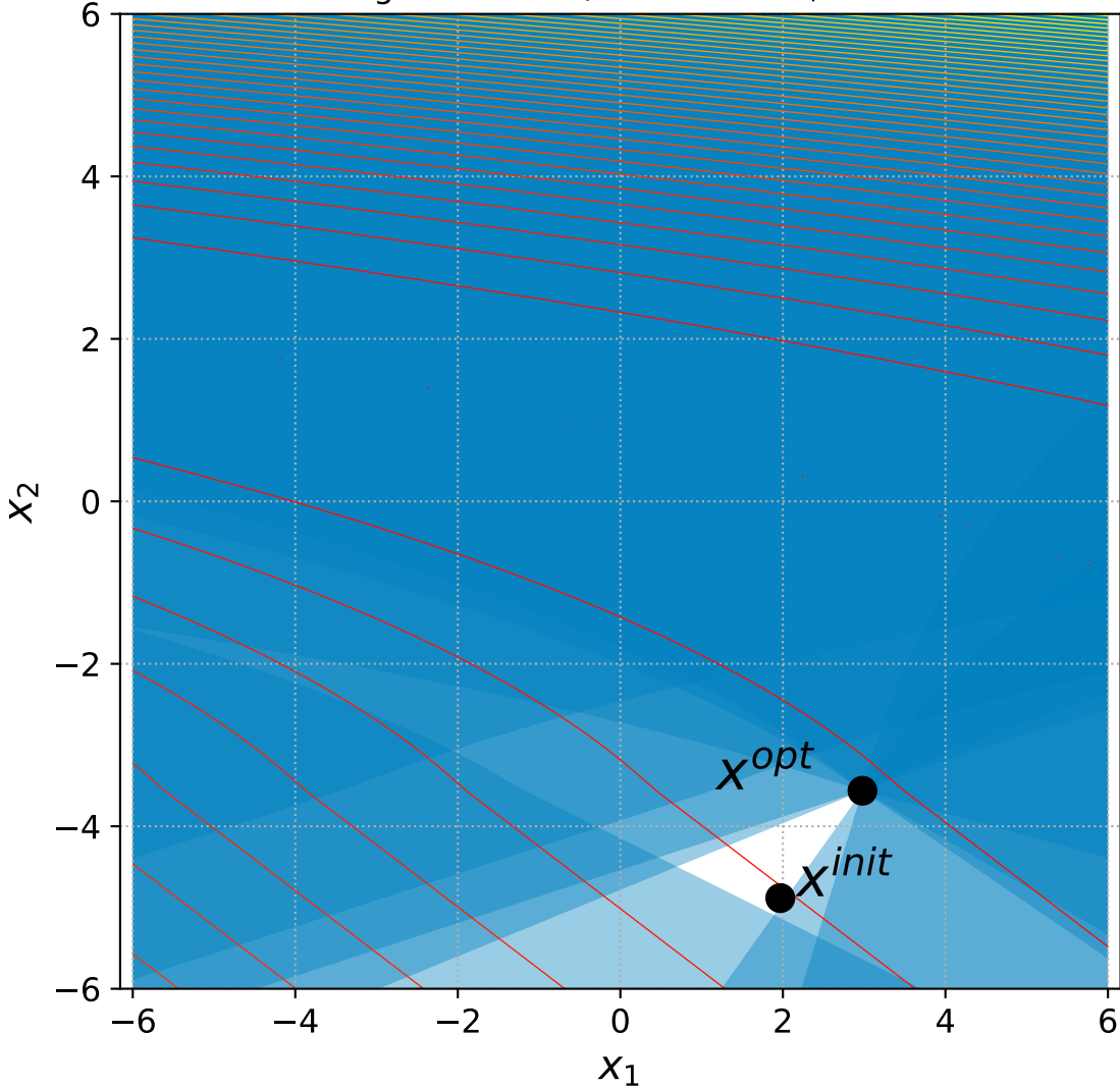
34 Bent Cigar with 6+n/2 constraints, instance=15
