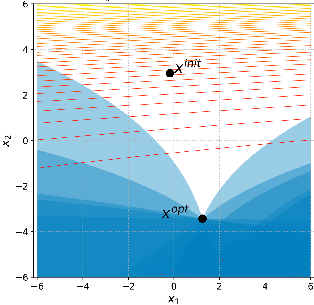
34 Bent Cigar with 6+n/2 constraints, instance=13
