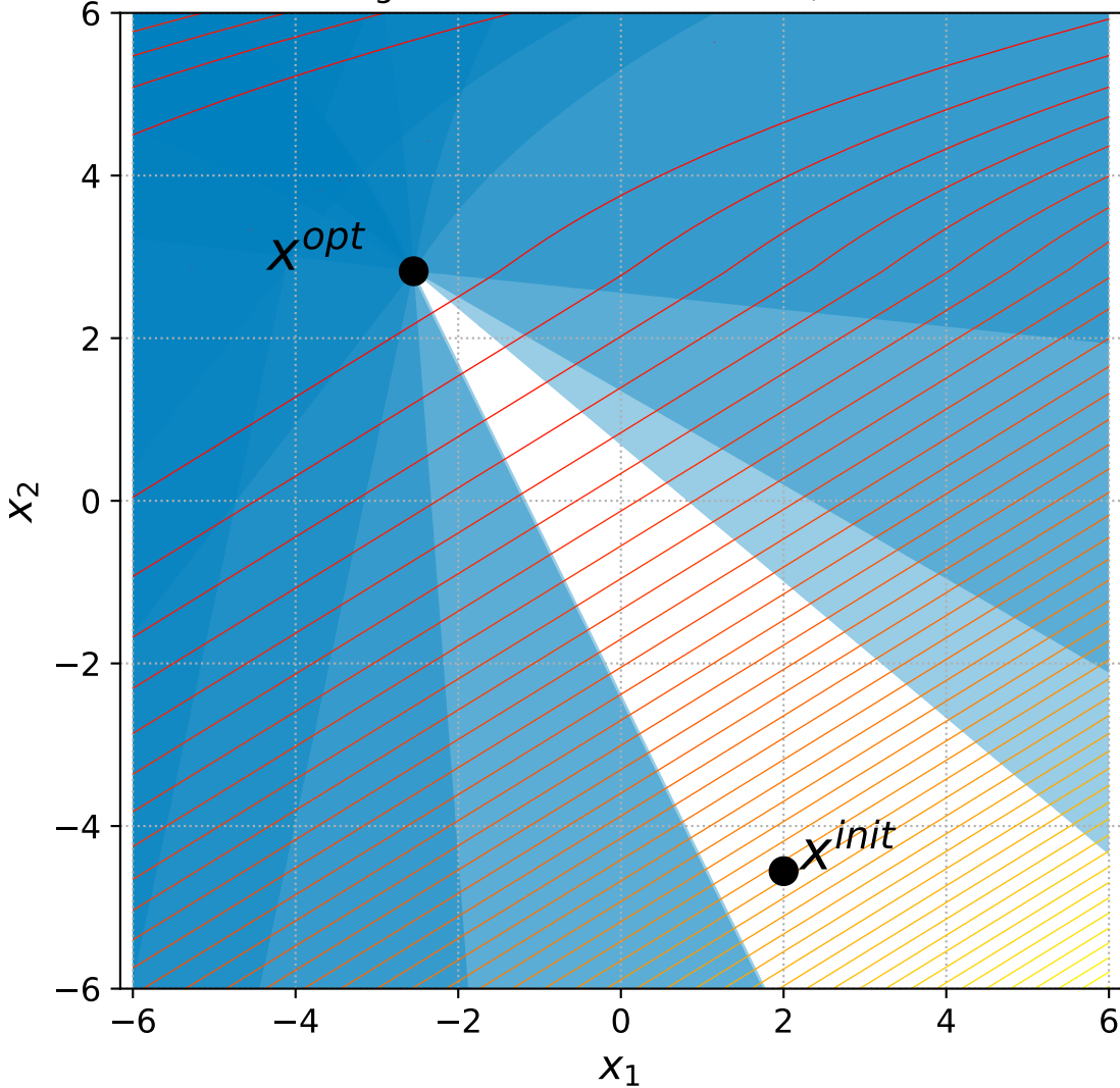
34 Bent Cigar with 6+n/2 constraints, instance=12
