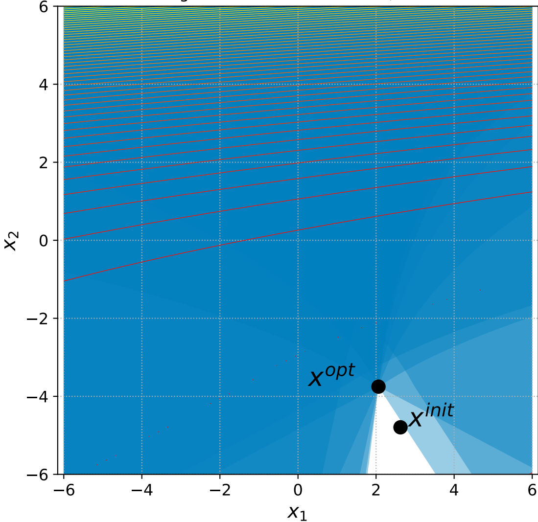
34 Bent Cigar with 6+n/2 constraints, instance=11
