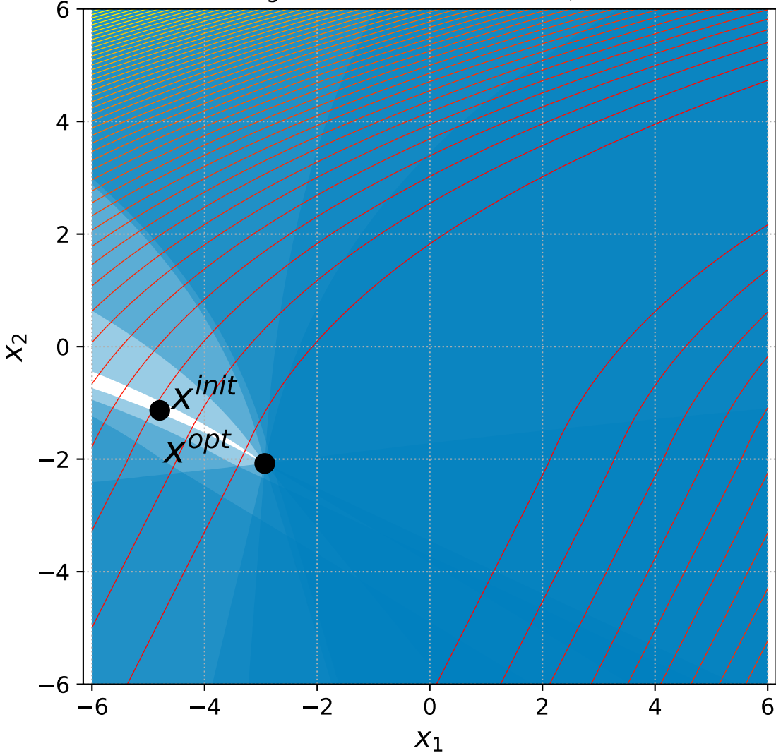
34 Bent Cigar with 6+n/2 constraints, instance=9
