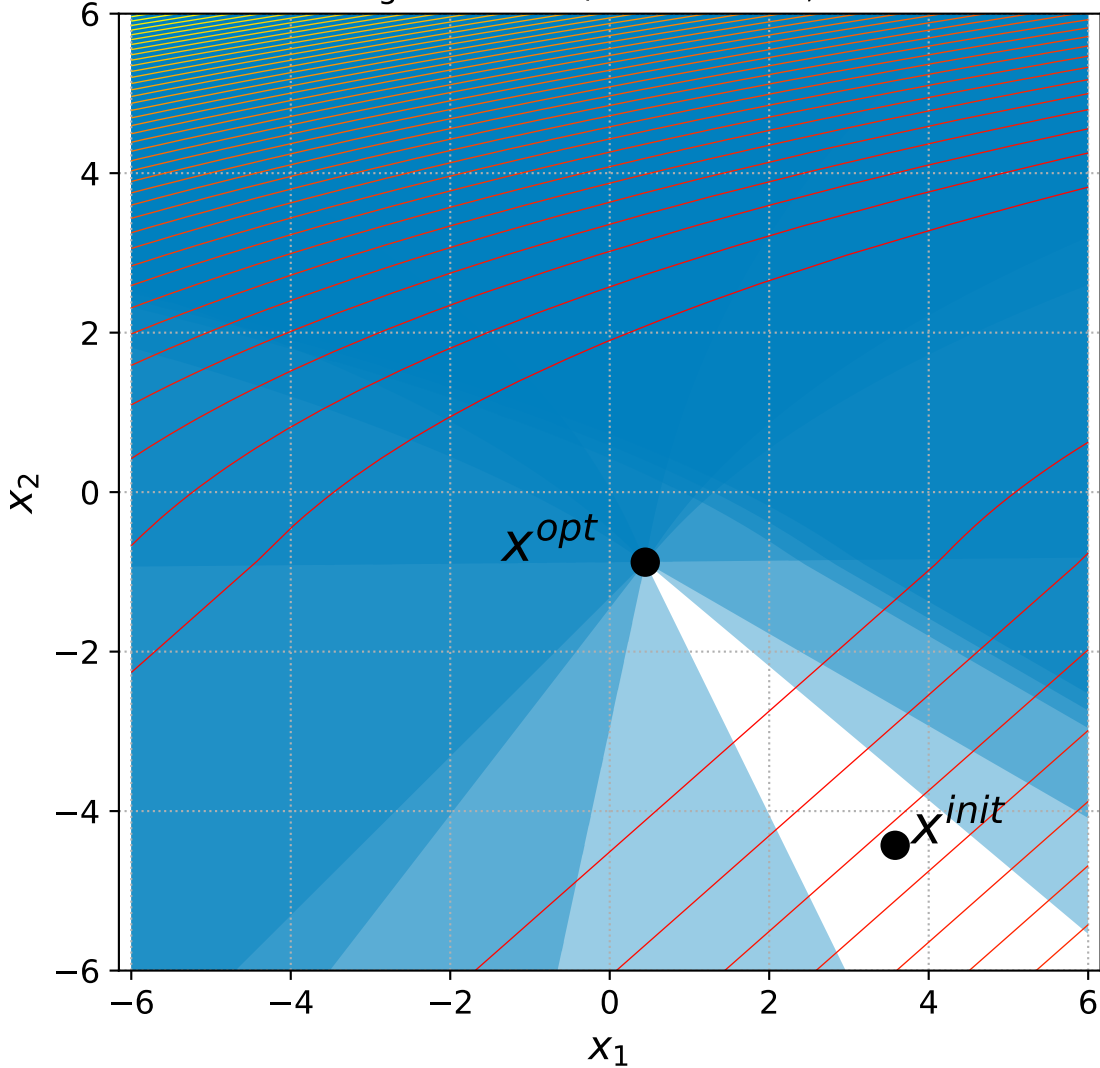
34 Bent Cigar with 6+n/2 constraints, instance=7
