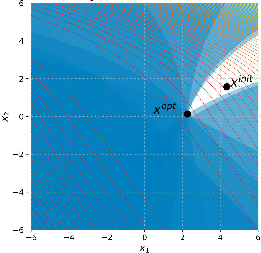
34 Bent Cigar with 6+n/2 constraints, instance=6
